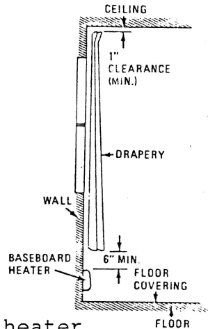
EXAMPLE Positioning Drapes Near Heater
